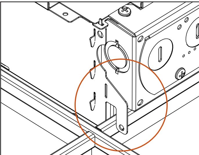
5 Tabs should rest on grid as shown
