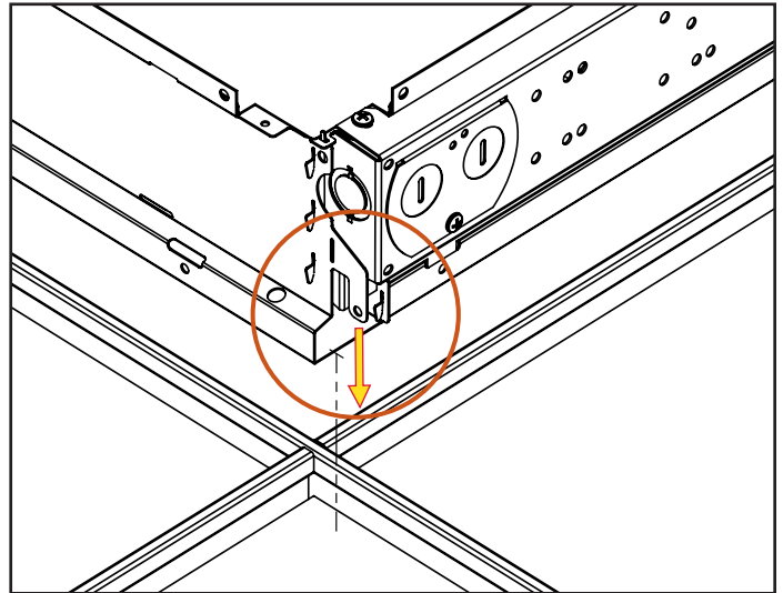
4 Make Sure Tabs are properly aligned
