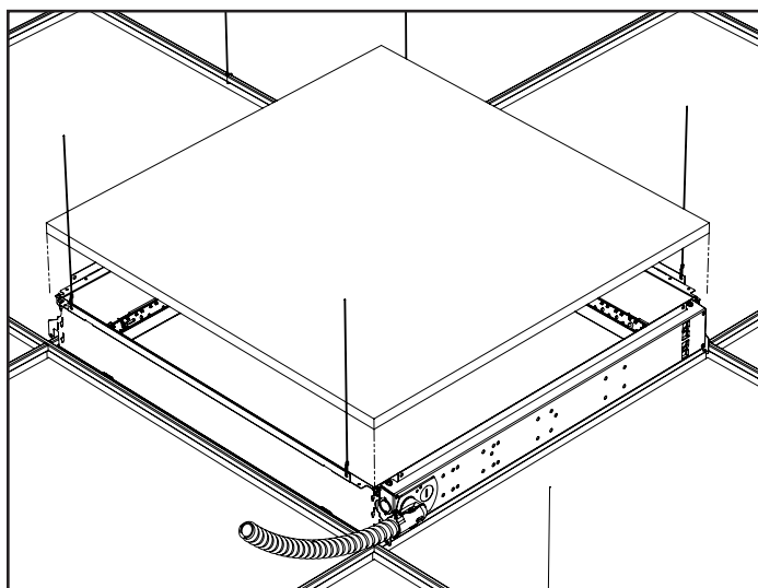
12 BRT only, place tile on top of the luminaire
