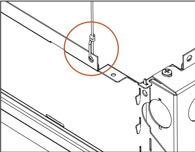
7 Secure fixture to structure with tie-wire on a all 4 corners (Detail)
