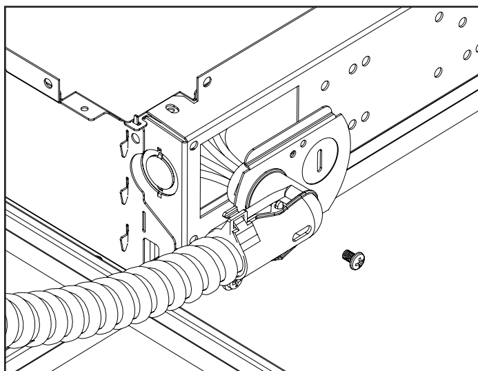
12 Push splice back into wire cavity and re-attach access plate
