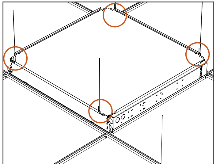
6 Secure fixture to structure with tie-wire on all 4 corners Tie wire by others
