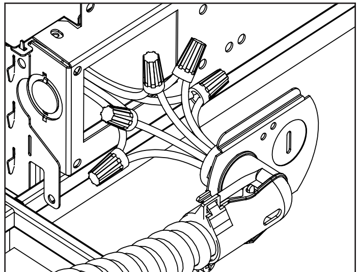
10 Attach flexible conduit to access plate and make wire connections
