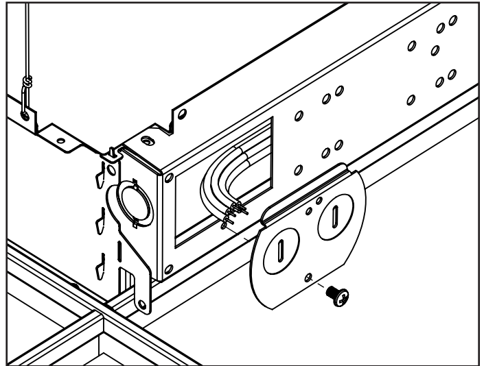
8 To make power connection remove screw and remove access plate and pull out wires
