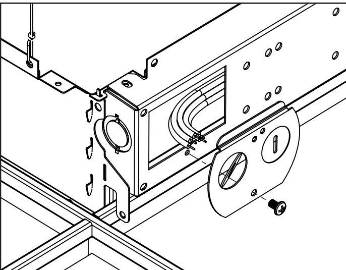
9 Remove 7/8" KO
