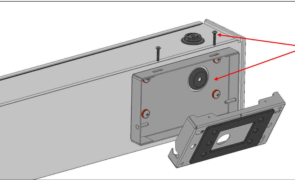
J-Box mounting screws located between mounting plates, remove two screws to access
