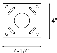
Mounting Plate (Gasketed)
