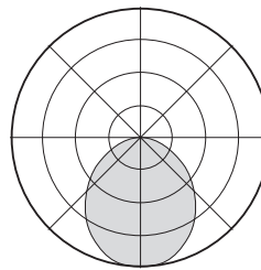
PXP2-F 100% Direct Light Distribution
