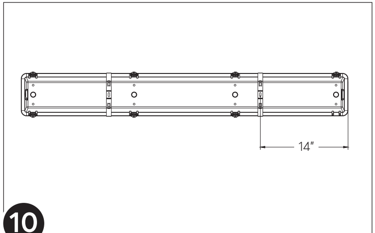
Mounting bracket centerline should be 14" from end of fixture
