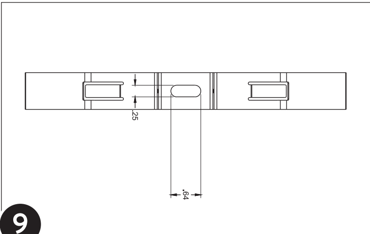
Bracket mounting hole dimensions
