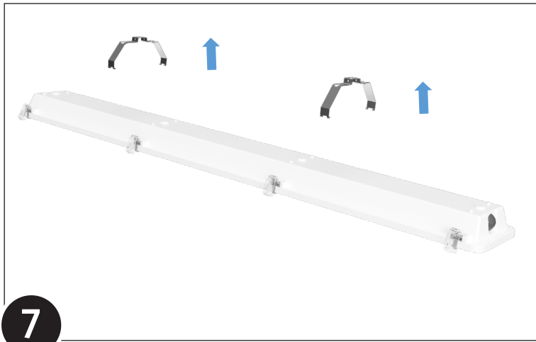
Mounting brackets removed
