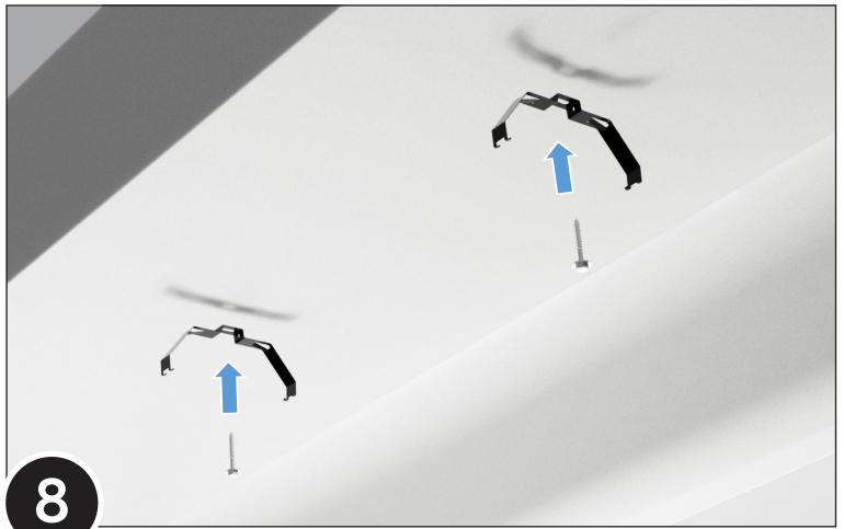
Mount brackets to building structure (hardware by others)
