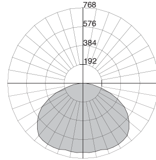
Cat.# SA-132T8...-SYM* Initial lamp lumens - 2900
