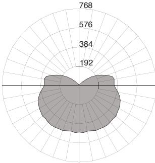
Cat.# SA-132T8...* Initial lamp lumens - 2900
