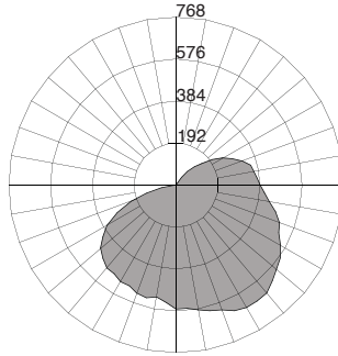
Cat.# SA-132T8...-ASY* Initial lamp lumens - 2900
