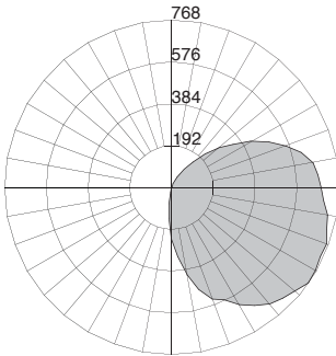
Cat.# SA-132T8...-RASY* Initial lamp lumens - 2900
