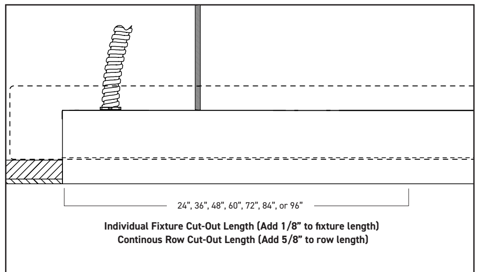
RT1 fixture side view
