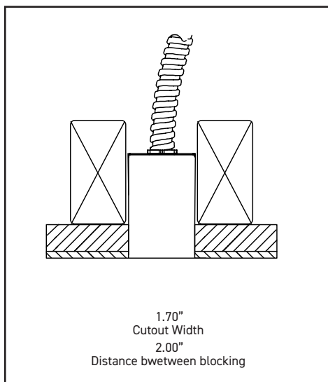
RT1 fixture end view
