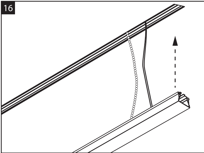
Replace the lens/LED board assembly from the bottom of the luminaire. Repeat for all fixture in the row.
