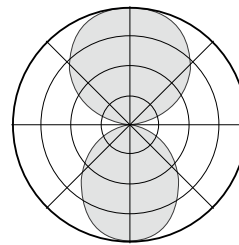
RP13-B (White Baffle) 36% Downlight / 64% Uplight
